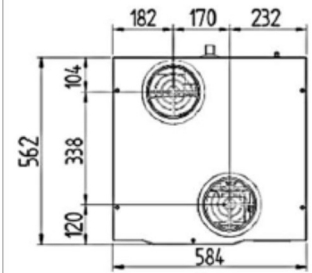
Figure 3. Dimensions, mm
