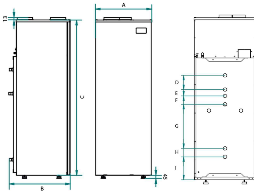
Figure 3. Dimensions, mm
