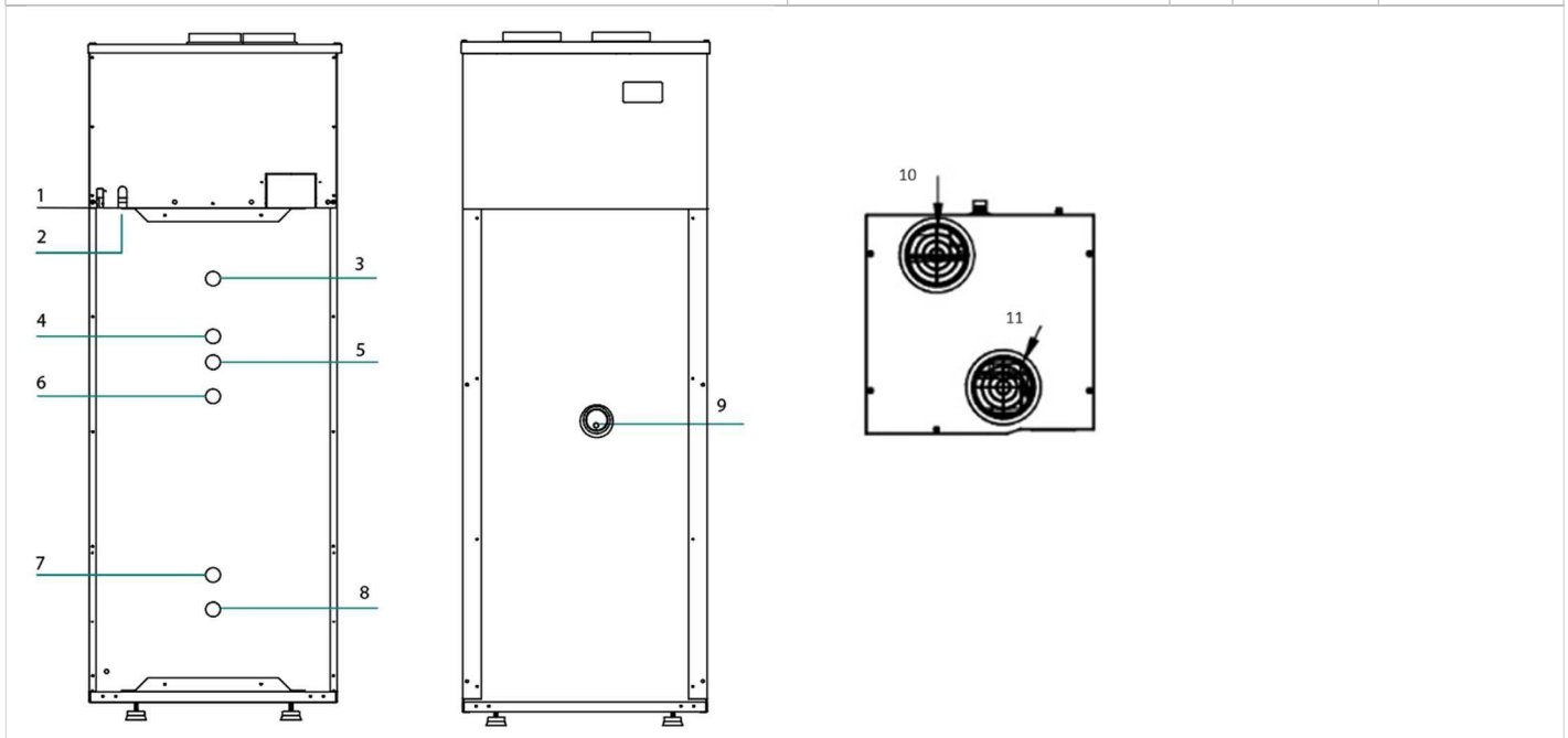
Figure 4. Back connections
