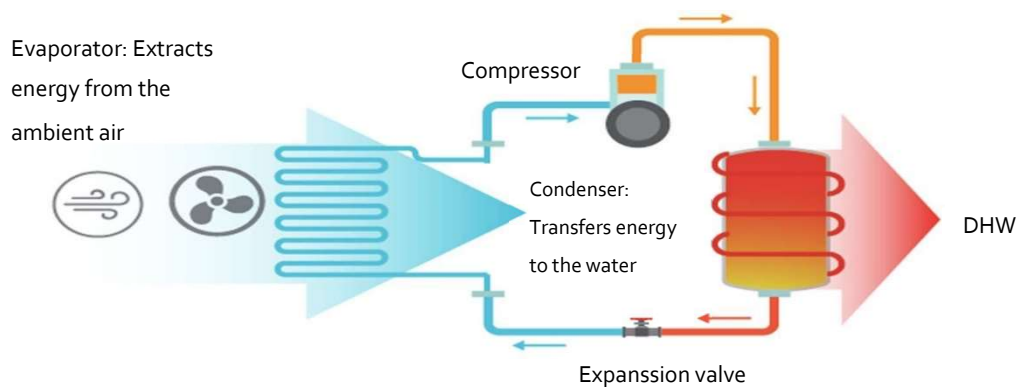
Figure 1: Operating principle
