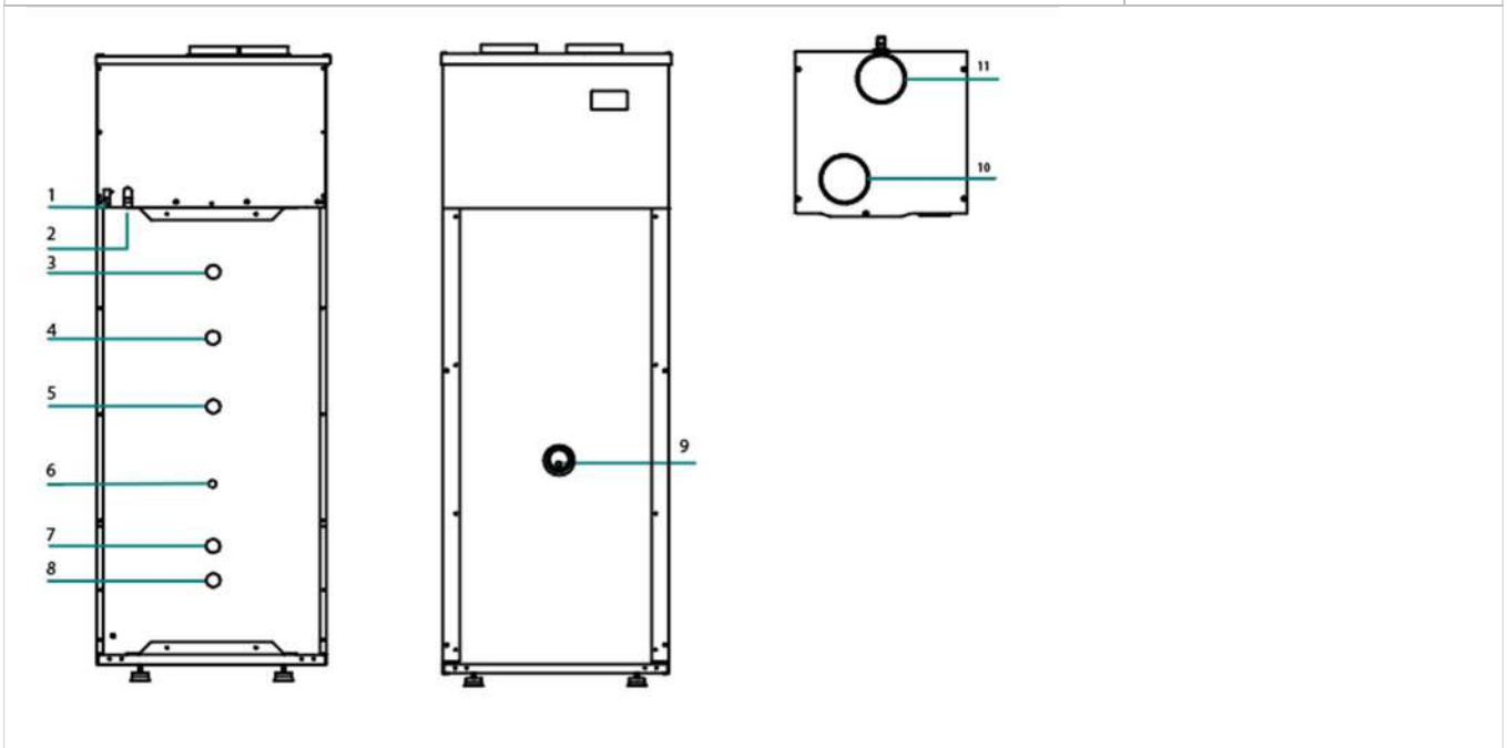
Figura 4. Back connections
