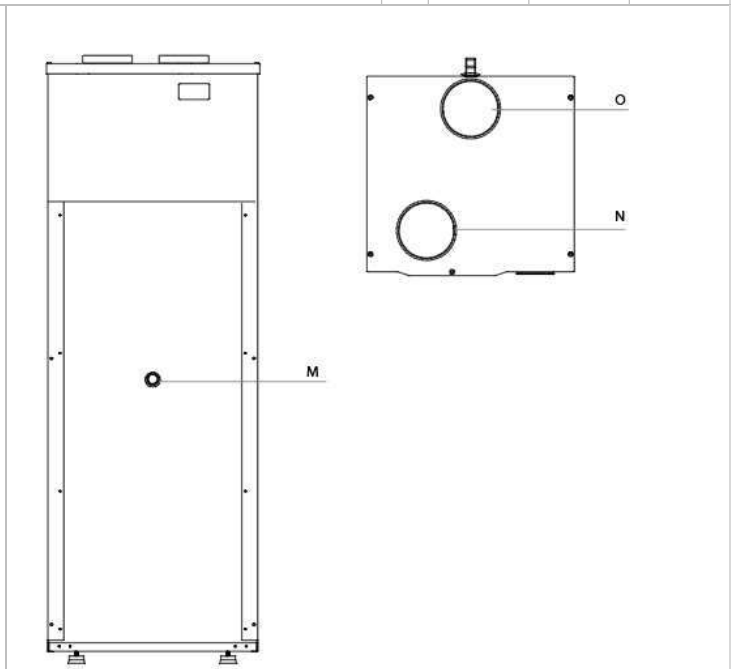
Figure 5. Front connections
